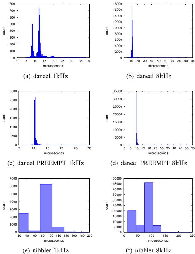
Fig. 3. Histograms of Ach messaging latencies. Daneel is a Core 2 Duo running Ubuntu 10.4. The PREEMPT version used the RT_PREEMPT kernel patch. Nibbler is an 800MHz ARM CPU running Debian 6.0.
