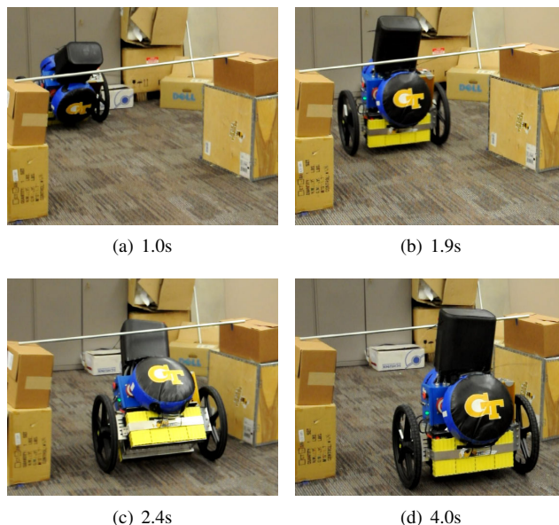
Fig. 1. A two-wheeled robot executing the hand-tuned hybrid limbo motion.
